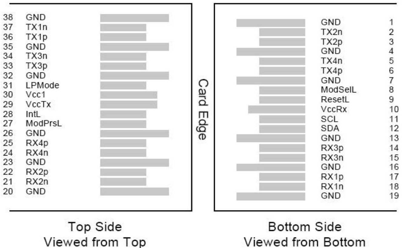
Figure 2: PT-40G-SR4-85 Transceiver Electrical Pad Layout
