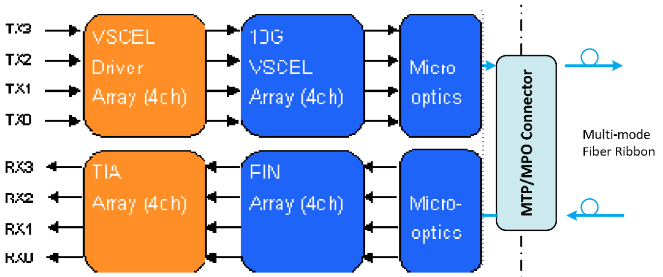
Figure 1: PT-40G-SR4-85 Transceiver Block Diagram
