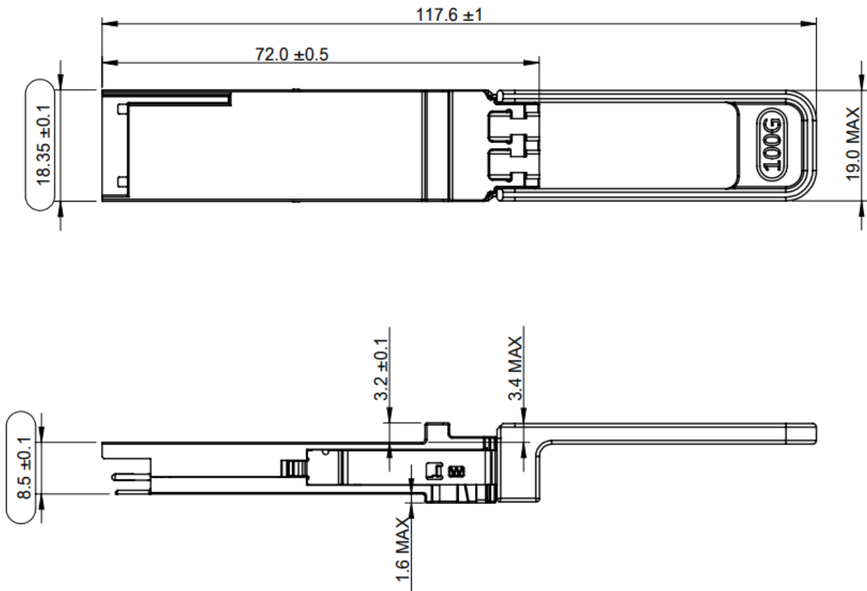
Figure 4. Mechanical Outline
