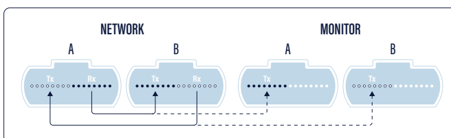
F4M4-SR8 TAP DIAGRAM
