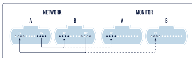
F4M4-SR4 TAP DIAGRAM
