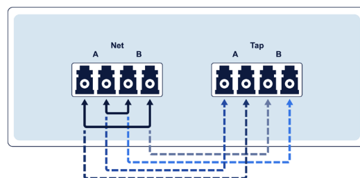
BiDi TAP internal port connectivity
